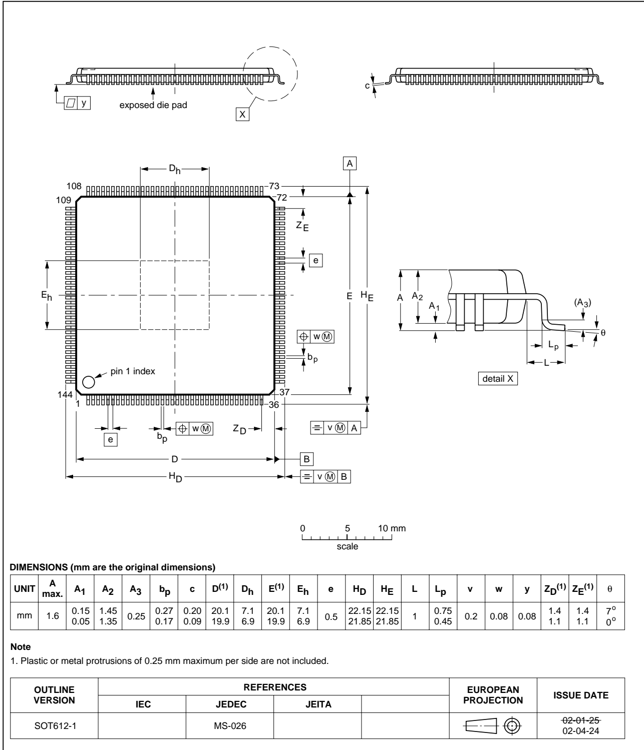
Fig 19. Package outline.
