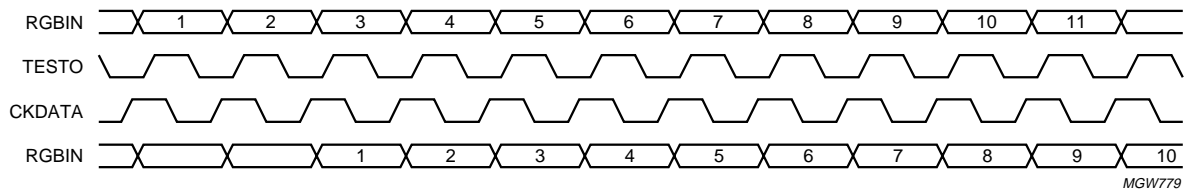
Fig 11. Timing diagram; single port mode (Dmx = 0).
