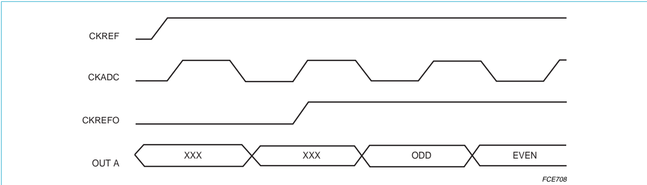
Fig 7. Definition of odd and even pixels; Edge = 0, Dmx = 0 and Ckrp = 1.
