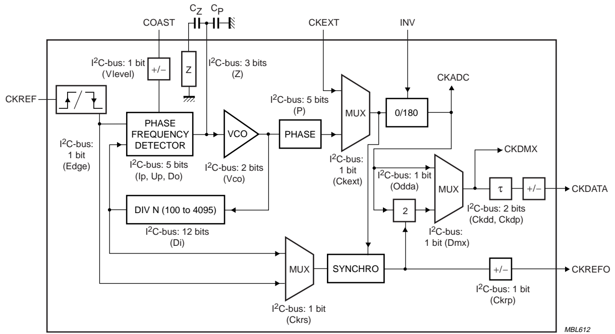
Fig 3. PLL diagram.
